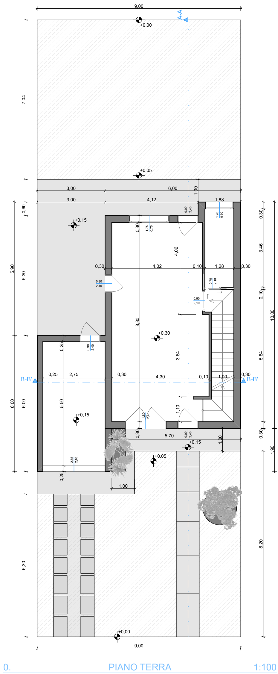
0. PIANO TERRA 1:100
